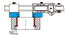
Measuring internal groove diameter with spherical measuring face (depth h2 \leq 0.295" )
