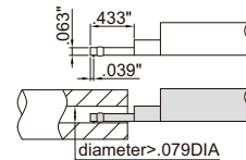
deep groove probe (optional), Part No. ISR-C002-DGP
