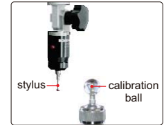
probe (optional), includes Ø2mm/.079" DIA and Ø3mm/.118" DIA styli, Ø25mm/.984" calibration ball, measuring accuracy is .0004"
