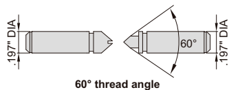
60° thread angle
