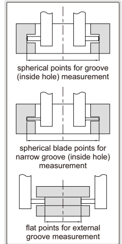
measure internal and external grooves
