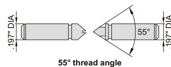
55° thread angle
