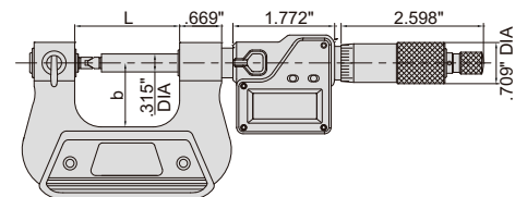
accuracy of micrometers with tips
