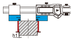
Measuring external groove diameter with flat measuring face (depth h1 \leq 0.98" )
